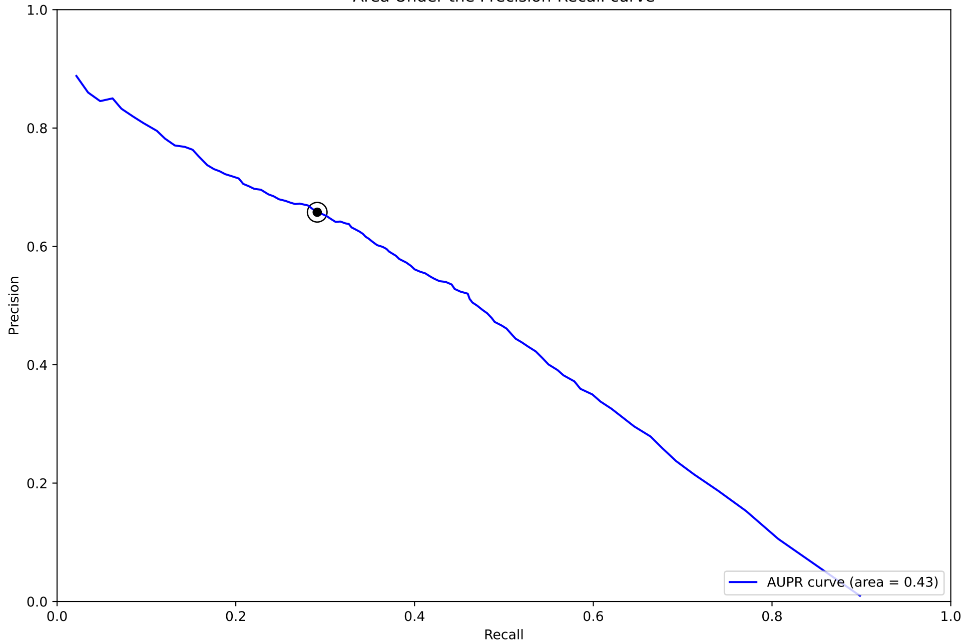
Area Under the Precision-Recall curve
